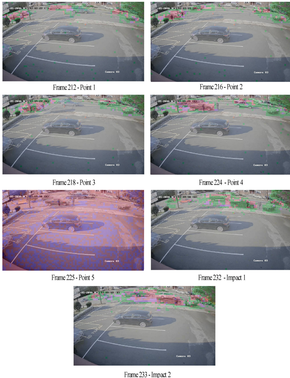
FIG. 2—Reverse projection roadway marking. [Color figure can be viewed at wileyonlinelibrary.com ]
