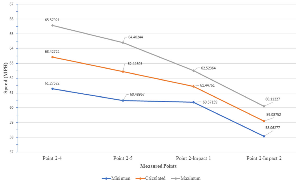
FIG. 4—Average calculated speed from point 2 with margin of error (in MPH). [Color figure can be viewed at wileyonlinelibrary.com ]
