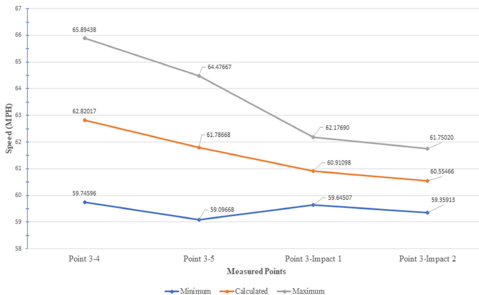
FIG. 5—Average calculated speed from point 3 with margin of error (in MPH). [Color figure can be viewed at wileyonlinelibrary.com ]
