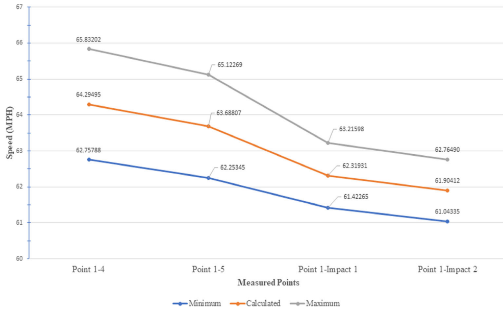
FIG. 3—Average calculated speed from point 1 with margin of error (in MPH). [Color figure can be viewed at wileyonlinelibrary.com ]
